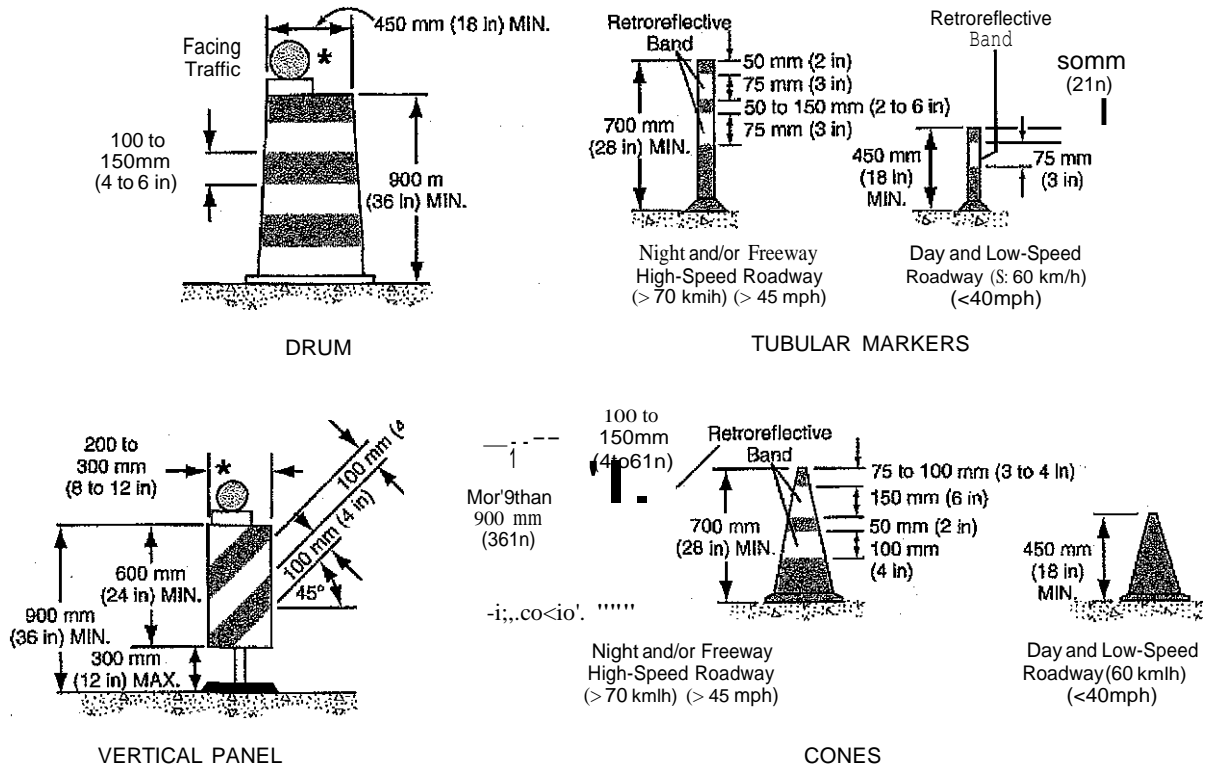
Figure 6F-7. Channelizing Devices (Sheet 1 of 2)
